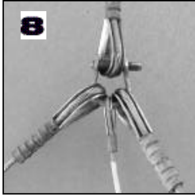
I-17 Pigtail/Forestays
